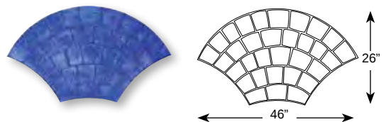
European Fan, FM-650 S/O 26" x 46" (66.04 x 116.84 cm) Blue Matching skin/touch-up wheel: Smooth Slate/ FM-6520 Joint size 1/4"-1/4" wide, 3/8" deep Stone size 3 3/4"-5 1/2" wide, 4"-6 1/2" long
