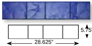
London Cobble Strip, FM-560 S/O 5.75" x 28.625" (14.605 x 72.71 cm) Blue Matching skin/touch-up wheel: Slate/ FM-6510 Joint 1/4"-1/4" wide, 1/4" deep Stone size 5 1/2"-5 3/4" wide, 5 1/4"- 8" long
